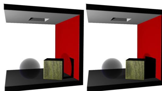
Figure 5: Different error values for deep shadow mapping: 0.00005 (left), 0.01 (right). Artifacts appear when using too small error values.
