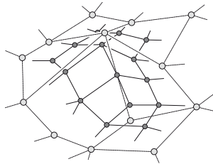
Figure 1: A step in the Catmull-Clark subdivision scheme.
