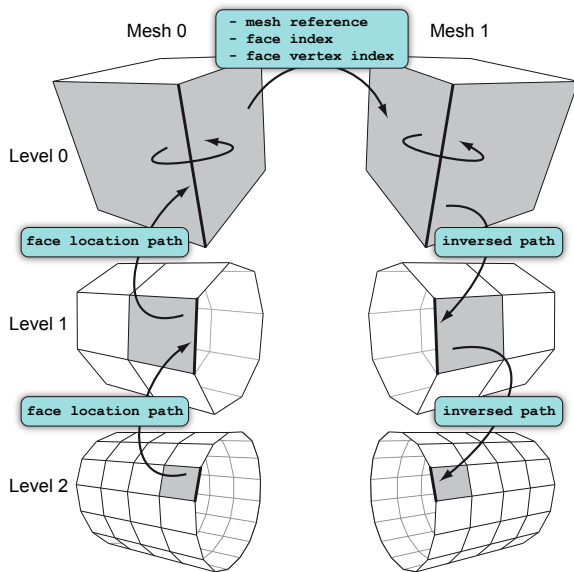
Figure 5: Traversing the subdivision hierarchy along the face location path.
