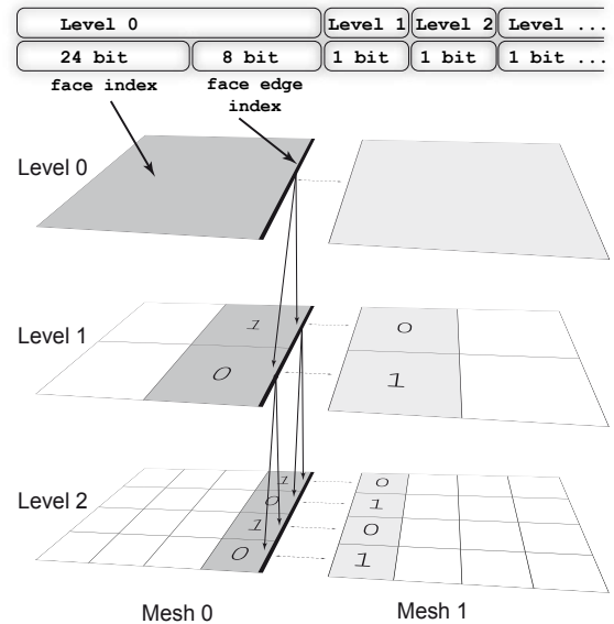
Figure 4: Encoding the subsequent face location path along a stitch edge.
