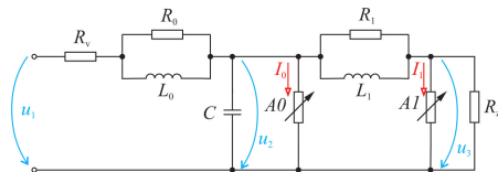
Fig. 1. Electric circuit model used for IEEE arrester
