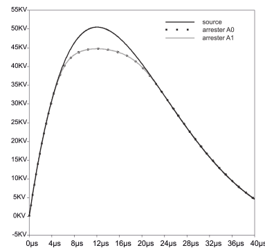
Fig. 3. Comparison of the results from LTSpice
