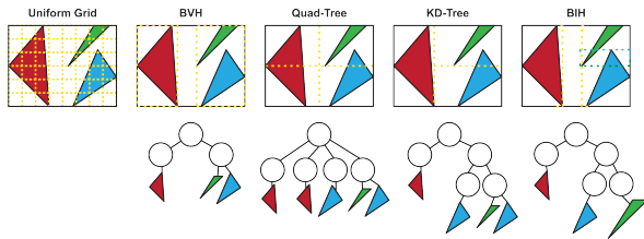
Figure 1: 2D examples of Acceleration Structures.
