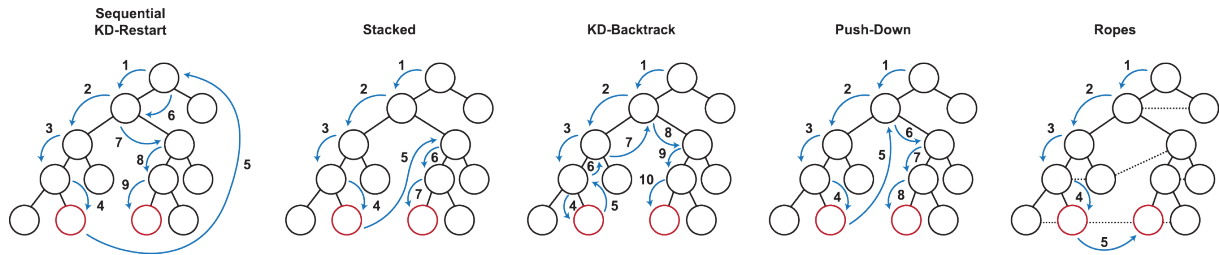
Figure 2: Traversal order example for different KD-Tree Traversal algorithms. The red circles represent two leaf nodes that, must be traversed in order. The main difference between KD-Tree traversals is how they go from the red circle to the other. The dashed lines represent the ropes.
