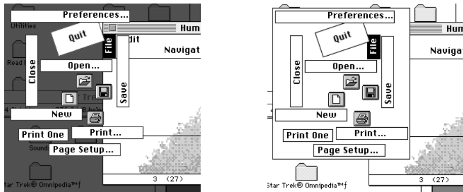
Figure 4: Two possibilities to emphasize menu items and the related buttons.
