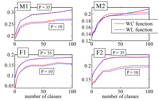
Fig. 3. Dependency between number of classes and P_{LSF} for particular speakers. Parameter order was set to 10 and 35.
