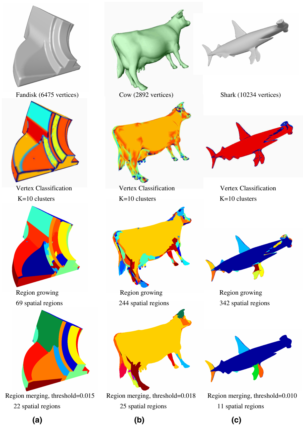
Figure 11. Segmentation of (a) Fandisk, (b) Cow and (c) Shark object. The number of curvature clusters is 10 for all. The region merging threshold is 0,015 for Fandisk, 0,018 for Cow and 0,010 for Shark.
