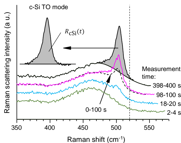
FIG. 1. Selected Raman spectra recorded in 2 s periods at different times (laser power 8.5 mW). Reference c-Si TO mode peak position 520\text{ cm}^{-1} is indicated. The dashed spectrum marks a long-time spectra acquisition. Note that lines were vertically shifted for better clarity. The inset shows extracted c-Si TO mode.
