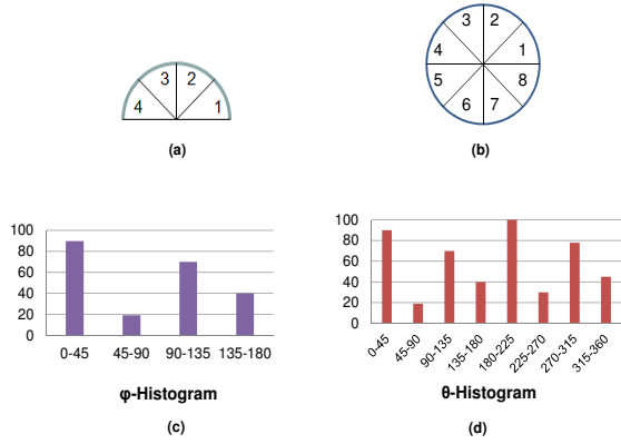
Figure 4: (a)Illustrative example showing 4 angular bins for \phi . (b)Illustrative example showing 8 angular bins for \theta . (c)-(d)Sample \phi - Histogram and \theta - Histogram for a cell.
