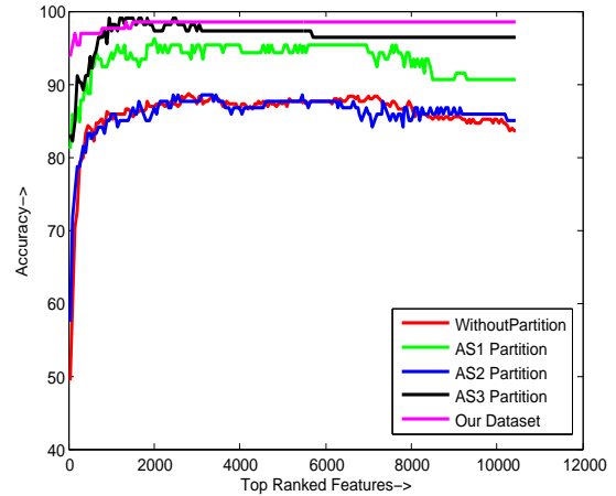
Figure 9: Recognition accuracies using different number of top ranked features.
