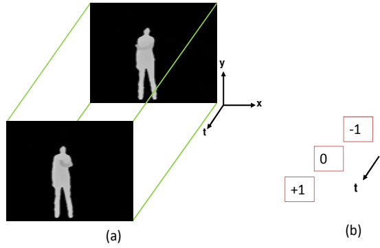
Figure 1: (a)Depth map sequence. (b)Gradient mask for a pixel along temporal domain.
