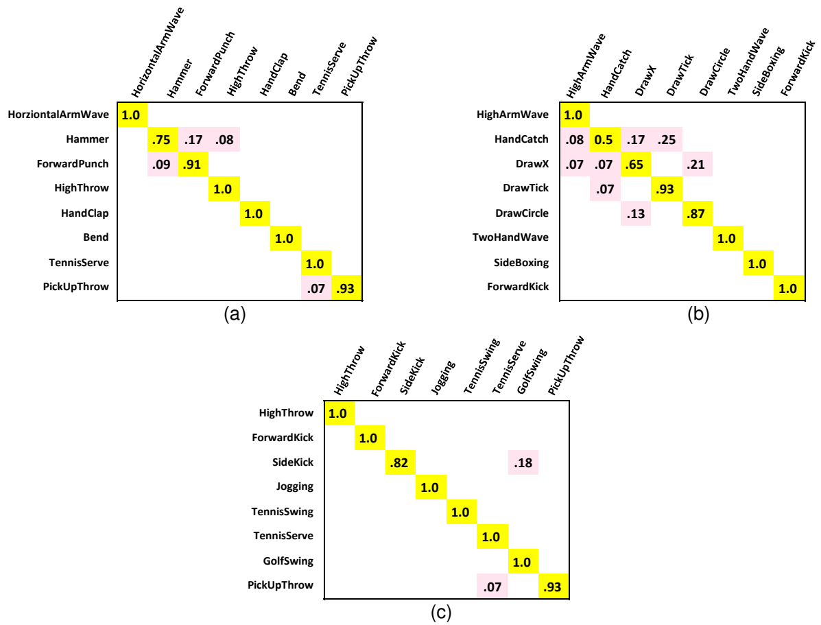
Figure 6: Confusion matrix for MSR Action3D Dataset. (a)AS1 (b)AS2 (c)AS3
