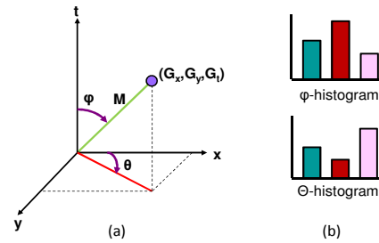
Figure 3: (a)Spherical coordinates for gradient of a pixel. (b) depthHOG in a cell.
