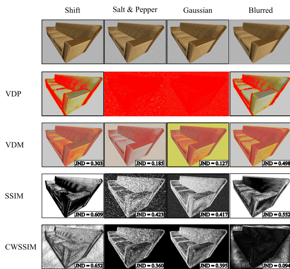
Figure 6: Objective quality metrics responses to shifted, salt & pepper and Gaussian noise contaminated and blurred images.
