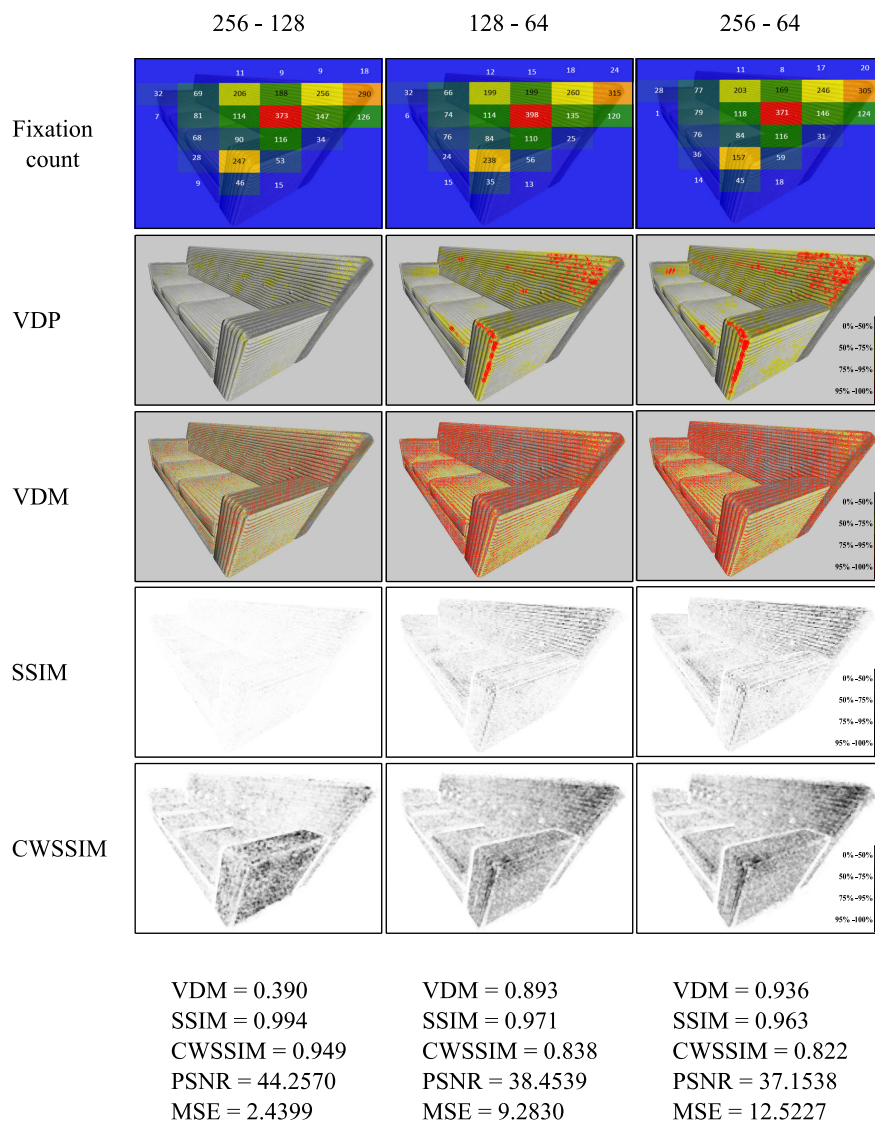
Figure 1: The output images of four IQMs by sofa with different 'Cord' texture resolution pairs. The color-scales on the right side indicate probability values of metrics in each pixel. The last row presents Just Noticeable Difference (JND) values of VDM, SSIM and CWSSIM. Additionally the MSE and PSNR, for each image pairs are also presented.
