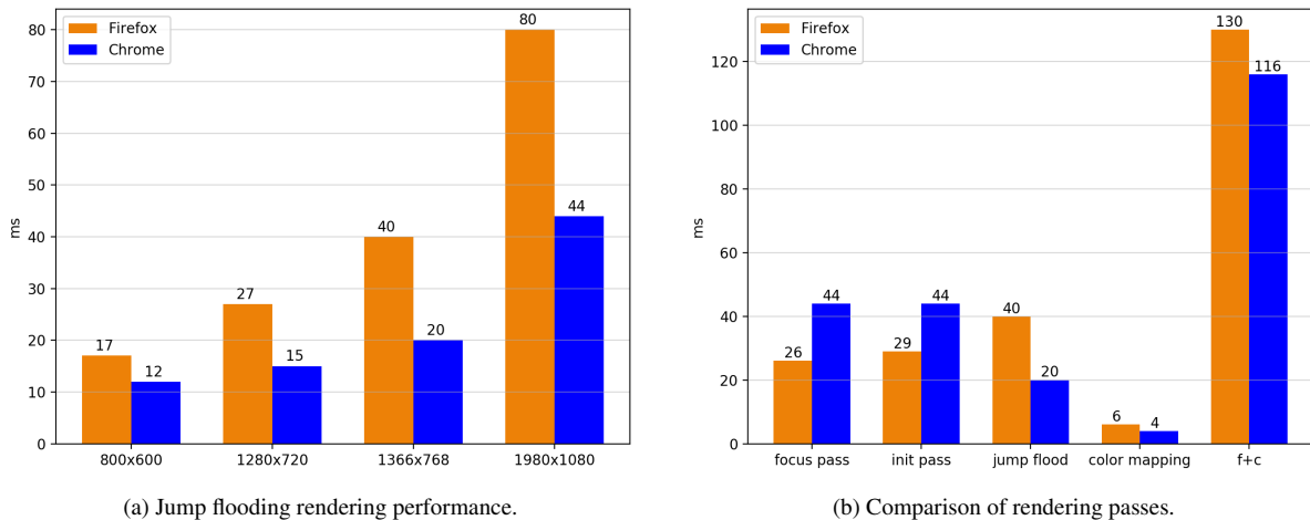
Figure 9: Measurement results of rendering performances with the browsers Mozilla Firefox and Google Chrome. Measurements are performed for (a) the jump flooding algorithm and (b) the rendering passes executed to create Focus and Context views. The performance is measured in milliseconds (ms).
