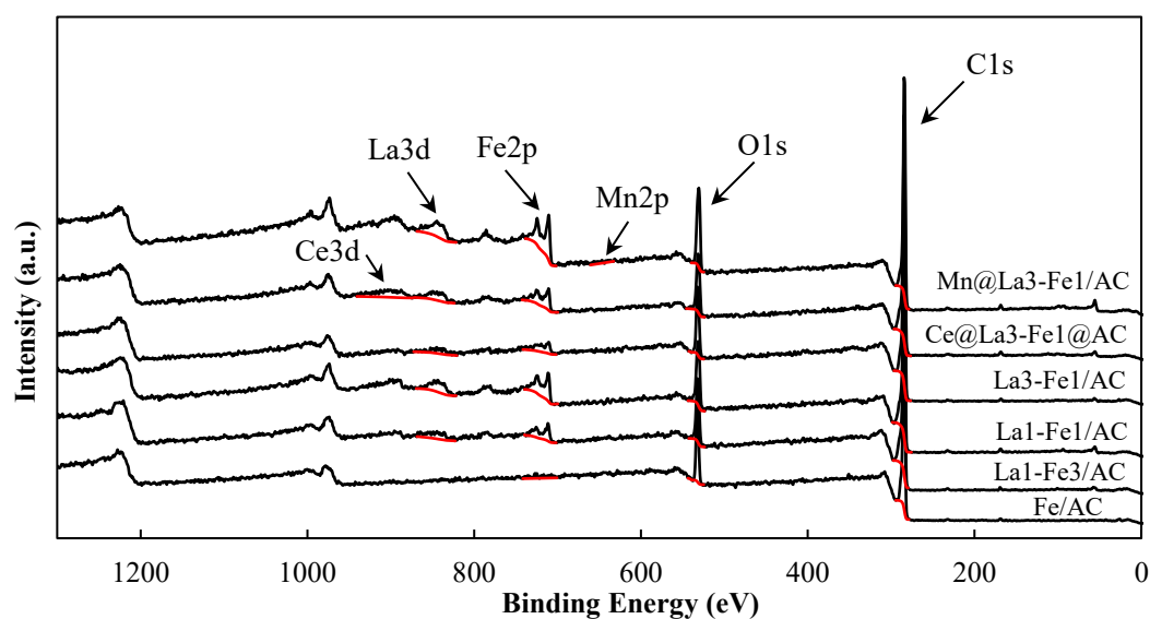
Figure 3. XPS survey spectrum of the synthesized catalysts.
