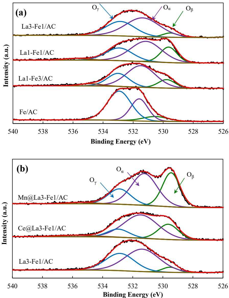
Figure 5. XPS spectrum of O 1s of the (a) \text{La}_3\text{-Fe1/AC} , \text{La}_1\text{-Fe1/AC} , \text{La}_1\text{-Fe}_3/\text{AC} , and \text{Fe/AC} , (b) \text{Mn@La}_3\text{-Fe1/AC} , \text{Ce@La}_3\text{-Fe1/AC} , and \text{La}_3\text{-Fe1/AC} .
