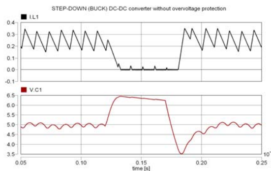
Figure 1. Spice simulation of a buck DC converter during sudden load change. Top - inductor current, bottom - output voltage
