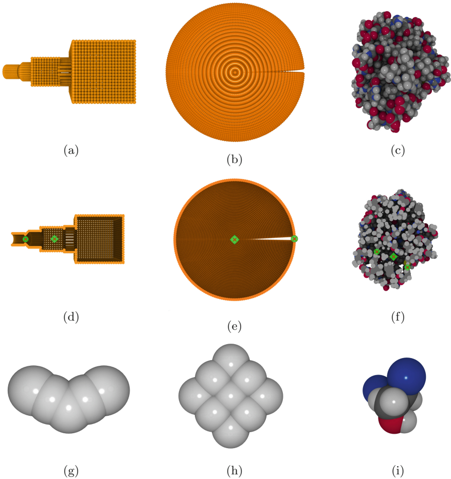
Fig. 3. (a-c) Tested data sets, (d-f) Cross-section through tested data sets, (g-h) Examples of navigated flexible agents (Color figure online)
