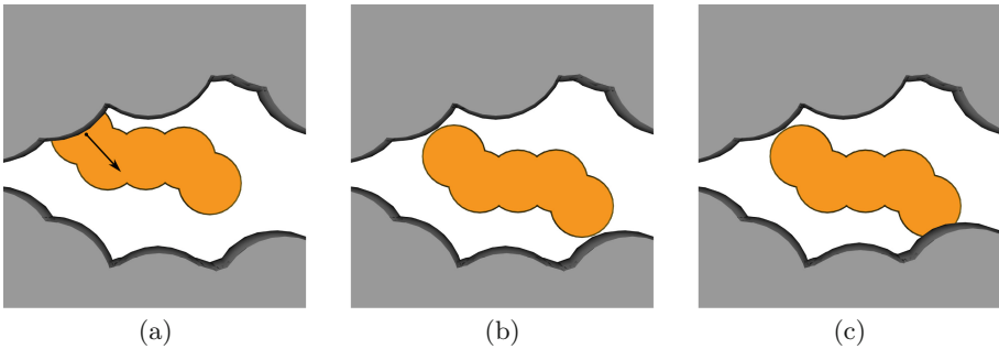
Fig. 2. (a) Small collision with obstacles, (b) Sample pushed correctly to the free space, (c) Sample pushed to another collision
