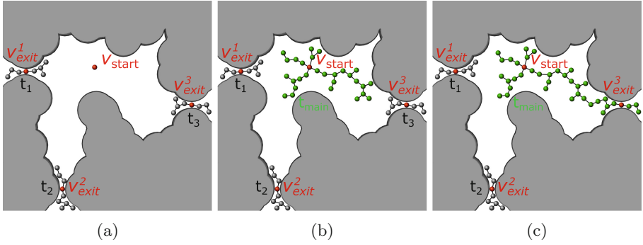
Fig. 1. (a) Sampling around exit points, (b) Sampling around the starting position v_{start} , (c) Merging exit point tree t_3 into the main tree t_{main}
