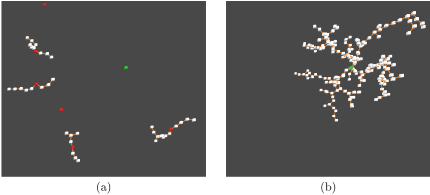
Fig. 4. Start of (a) The modified RRT algorithm with exit points, (b) Standard RRT algorithm
