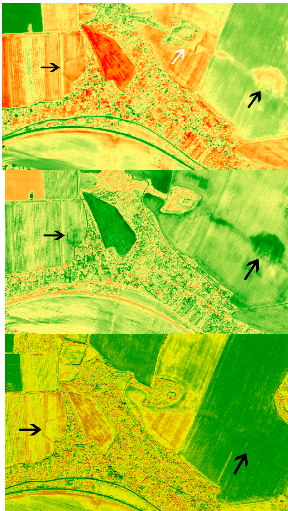
Figure 6. The linear defensive system composed of artillery forts in Třeboutice (district Litoměřice)—one semi-ruined (white arrow) and two completely buried (black arrows), as scanned on 3 May 2006 by QuickBird-2, displayed in the following spectral bands: top —NIR, center —Red, bottom —NRVI. The present author's project, University of West Bohemia.
